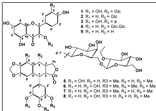
Figure 1. Phytoconstituents from P. hexandrum
