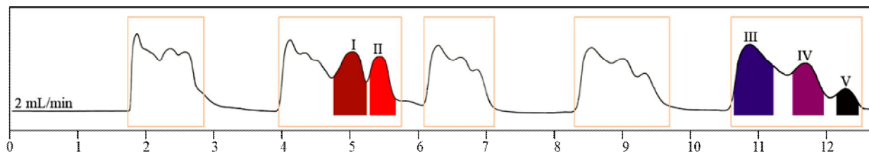
Figure 3. Offline-recycling HSCCC chromatogram for separation of compounds (1-5); Solvent system: HEMWat (1:9:4:6, v/v); Flow-rate: 2.0 mL/min; Detection wavelength: 254 nm; Rotation speed: 800 rpm; Separation mode: FWD-IN; 150 mg
