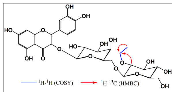
Figure 5. 2D-NMR correlations of compound 3
