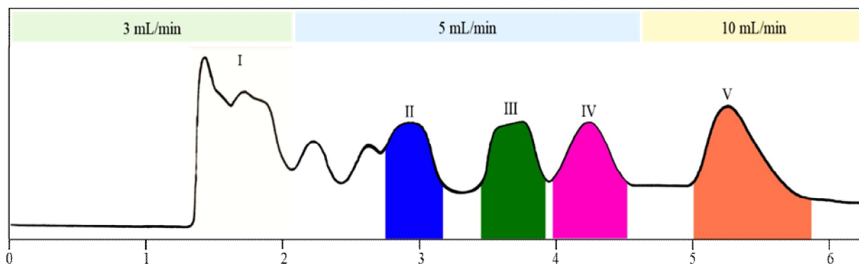
Figure 2. HSCCC chromatogram for separation of compounds from P. hexandrum ; Solvent system: HEMWat (1:9:4:6, v/v); Flow-rate: 3.0 mL/min for 125 min, 5.0 mL/min for 150 min, 10.0 mL/min for 110 min; Detection wavelength: 254 nm; Rotation speed: 800 rpm; Separation mode: FWD-IN; Sample loading: 300 mg
