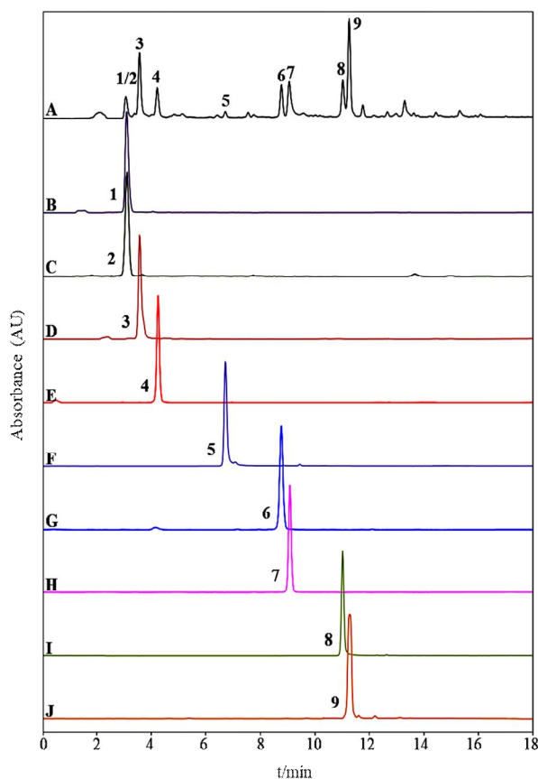
Figure 4. HPLC chromatograms of the crude sample and the isolated pure compounds. Experimental conditions: Waters Symmetry C_{18} column (5 \mu m, 4.6 mm \times 250 mm, i.d.); Mobile phase: acetonitrile and water; Flow-rate: 1.0 mL/min; Detection wavelength: 254 nm; Injection volume: 10 \mu L. A: crude (MeOH) extract; B-J: the isolated pure compounds (1-9)
