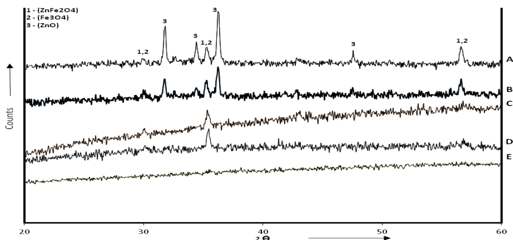
Figure 2. X-ray diffraction analysis of EAF dust sample. (A) untreated dust (B) 2 M alkali treated (C) 4 M alkali treated (D) 6 M alkali treated (E) 8 M alkali treated
