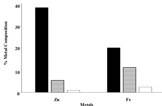
Figure 4. Metal composition % in residue with respect to concentrations 2M, 4M, 8M at 2h leaching time, 300 rpm and 90°C
