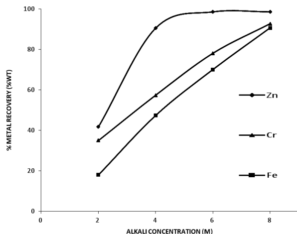
Figure 3. Recovery % of different metals vs. concentrations (at 2h leaching time, 300 rpm and 90°C)
