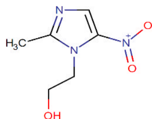
Figure 1. Metronidazole (MNDZ)
