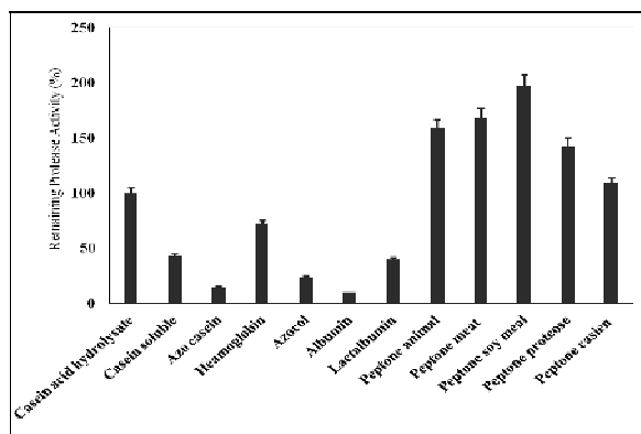
Figure 8. Substrate Specificity of purified protease activity of cotton seeds (Fraction-IV)
