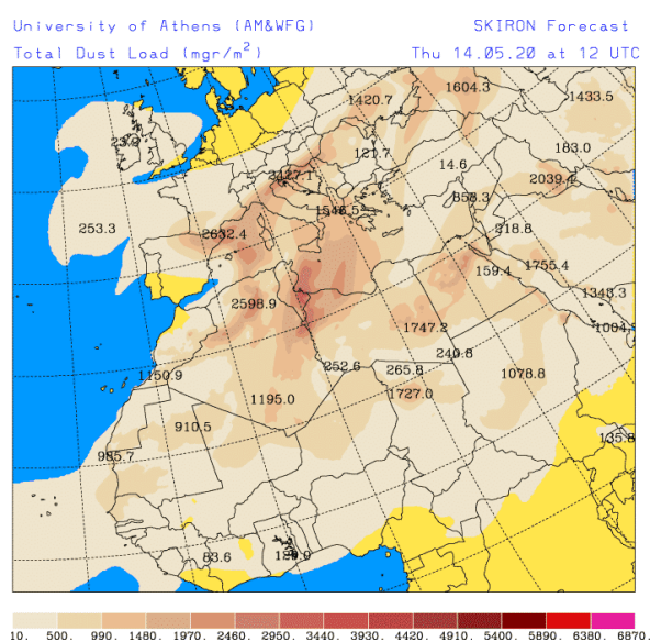
Figure 3. North African dust advection over Turkey
