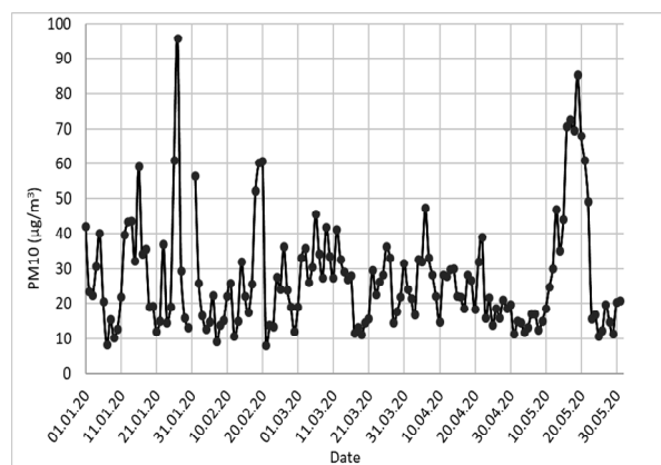
Figure 1. PM 10 values time series from January 1 to May 31, 2020
