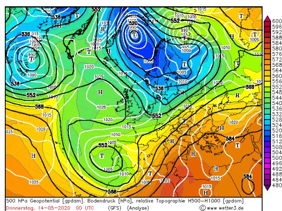
Figure 2. Strong advection of Saharan dust from North Africa into Europe during 14 May 2020
