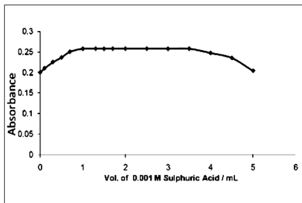
Figure 3. Effect of the acidity on the absorbance of Cu II -Sal-BH system.
