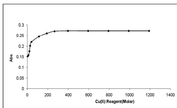
Figure 4. Effect of reagent on the absorbance of Cu II -Sal-BH system.
