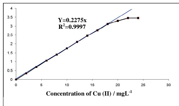
Figure 5. Calibration graph, 1-18 mgL -1 of copper(II).
