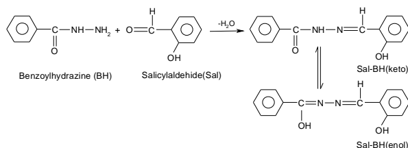
Reaction scheme of salicylaldehydebenzoylhydrazine(Sal-BH)
