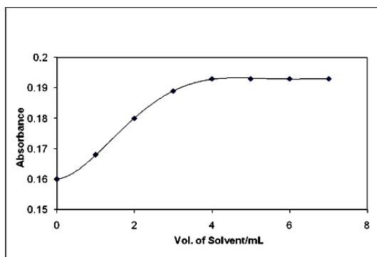
Figure 2. Effect of solvent on the absorbance of Cu II -Sal-BH system.
