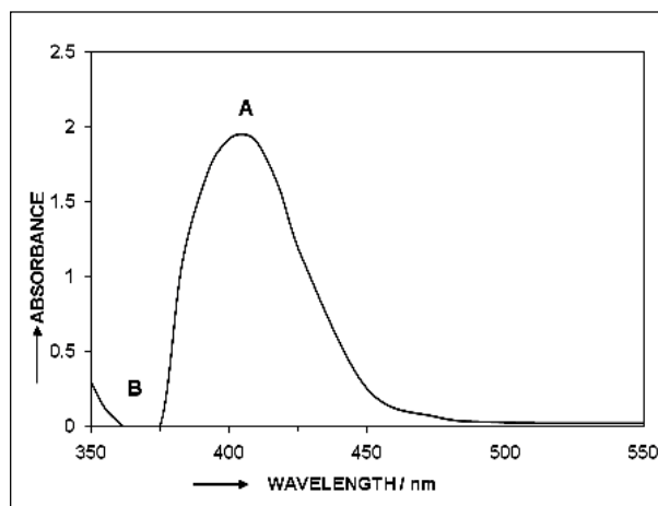
Figure 1. A and B absorption spectra of Cu II - Sal-BH system ( \lambda_{\text{max}} = 404\text{nm} ) and the reagent blank, respectively in aqueous solutions.
