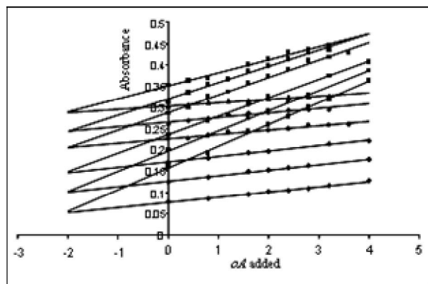
Figure 6. Plots of H-point standard addition method for fixed amount oA (2.0 μg ml -1 ) in the presence of 0.8, 1.6, 2.0, 3.2, 4.0 and 4.8 μg ml -1 of pA measured at (■) 480 nm and (♦) 610 nm.
