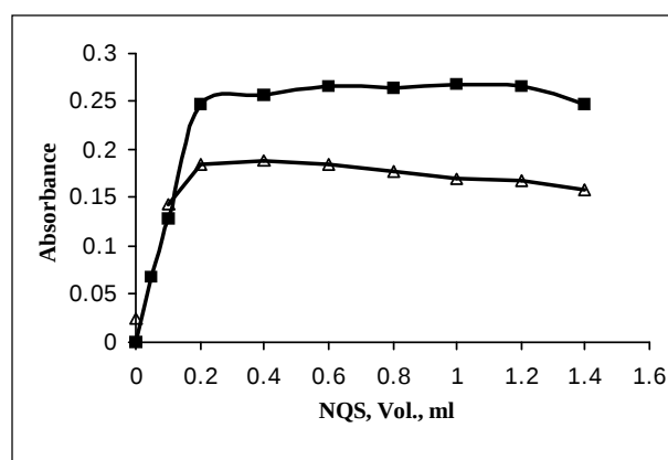
Figure 3. Effect of NQS reagent concentration on the absorption of reaction mixture of 4 \mu\text{g ml}^{-1} for each ( \Delta ) oA measured at 475 nm and ( \blacksquare ) pA measured at 495 nm in the presence of \text{Na}_2\text{CO}_3 solution.
