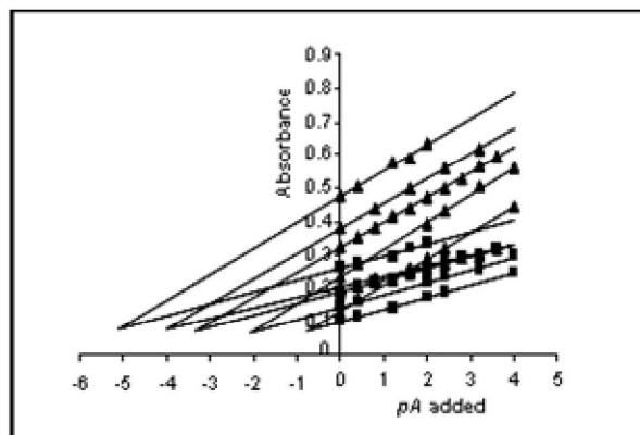
Figure 7. Plots of H-point standard addition method for fixed amount oA (2.0 μg ml -1 ) in the presence of 0.8, 2.0, 3.2, 4.0 and 5.0 μg ml -1 of pA measured at (♦) 531 nm and (■) 443 nm.
