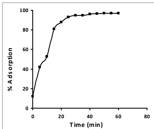
Figure-2. Effect of contact time time for the adsorption of endosulfan onto peach nut shells.
