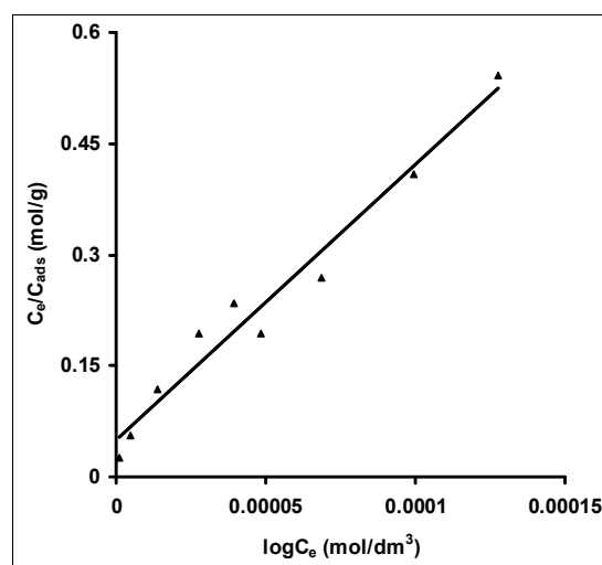
Figure-3. Langmuir adsorption isotherm of endosulfan onto peach nut shells.
