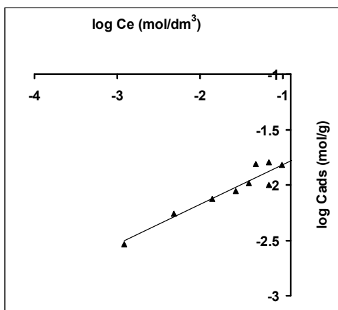
Figure-4. Freundlich adsorption isotherm of endosulfan onto peach nut shells.
