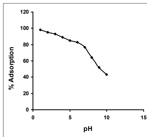
Figure-1. Effect of pH for the adsorption of endosulfan onto peach nut shells.
