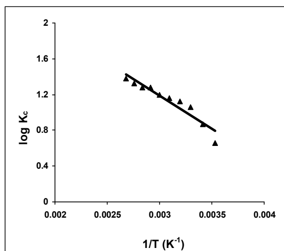
Figure-5. Effect of temperature on adsorption of endosulfan on peach nut shells.
