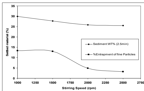
Figure 5. Effect of stirring speed on settling rate and % entrapment of fine particles (<10 µm) at 7.5 % Solids, 10.5pH, 5 min stirring time without dispersant.
