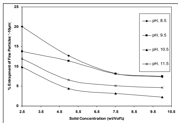
Figure 2. Effect of pH and solid concentration on stabilization of - 38 \mu m Dilband iron without dispersant.
