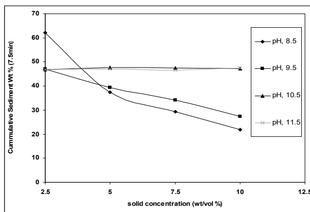
Figure 4. Effect of pH and solid concentration on settling rate after 7.5 min interval at 2500 rpm stirring speed, 5 min stirring time, and without dispersant.
