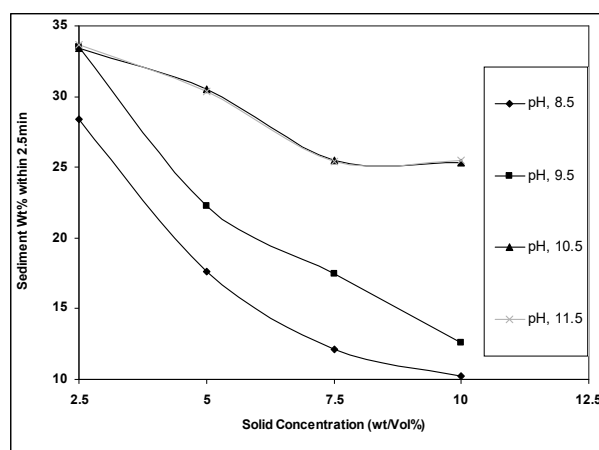
Figure 1. Effect of pH and solid concentration on stabilization of - 38 \mu m Dilband Iron ore slurry without dispersant addition.
