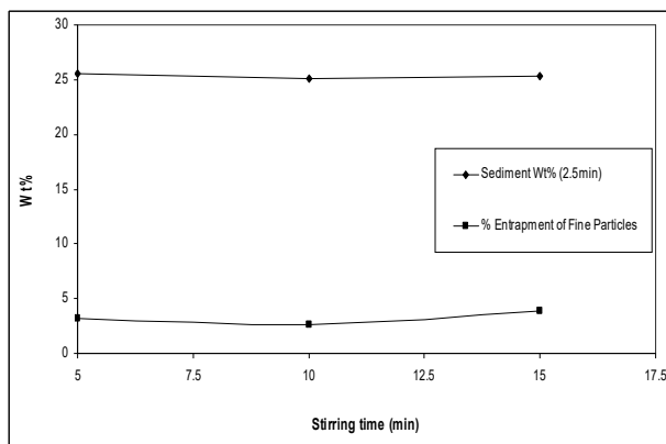
Figure 6. Effect of stirring time on stabilization of <38 µm Dilband iron slurry without dispersant.
