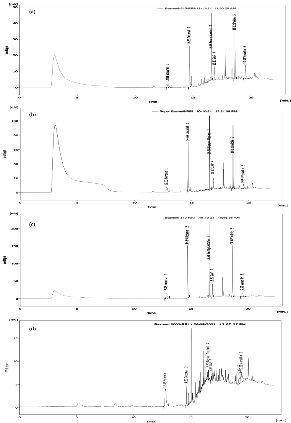
Figure 1. GC Chromatogram of (a) Basmati-515, (b) Super Basmati, (c) Basmati-370, (d) Basmati-2000
