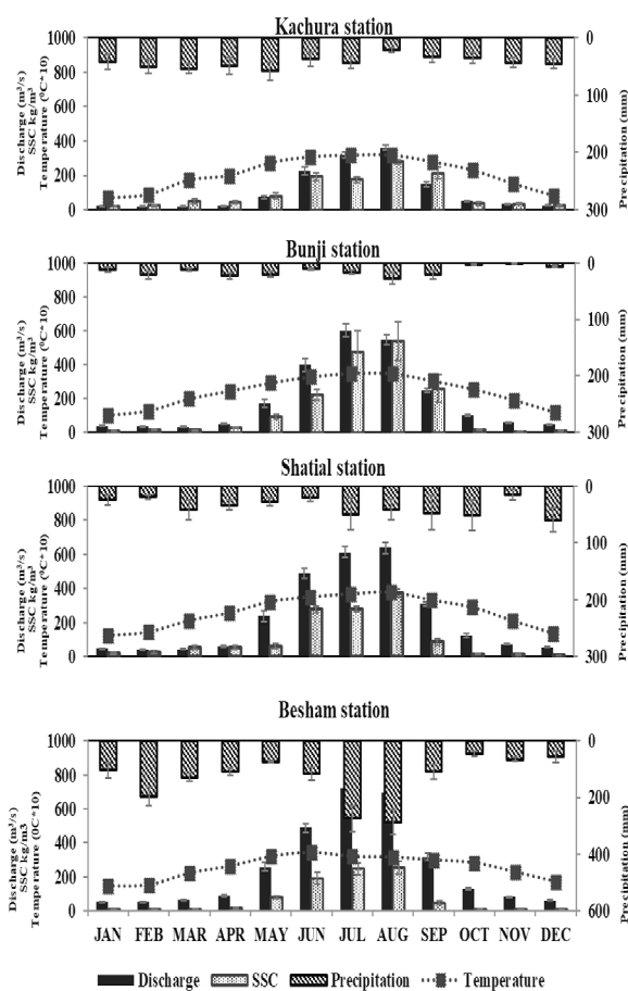
Figure 2. Mean monthly distribution of discharge ( \text{m}^3/\text{s} ), suspended sediment concentration (SSC) ( \text{kg}/\text{m}^3 ), precipitation (mm) and mean temperature ( ^{\circ}\text{C} \times 10 ) from 2005 to 2012 at four mainstream stations of the study area.
