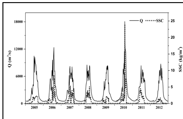
Figure 6. The hydrograph with sediment concentrations SSC ( \text{kg/m}^3 ) and discharge ( \text{m}^3/\text{s} ) at Besham Qila (Stretch-IV) from January 2005 to December 2012
