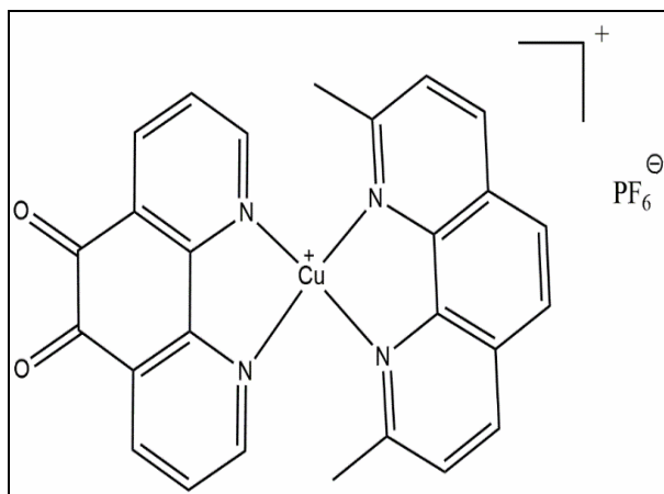
Figure 2. [Cu(I)(2,9-dmp)(phen-dione)]PF 6 (A2)
