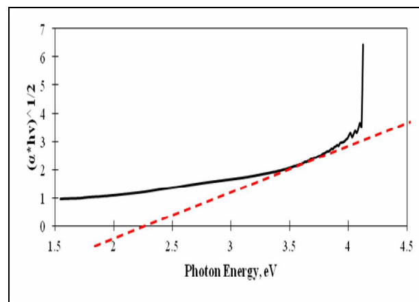
Figure. 5. Schematic diagram of Tauc plot used to measure the optical bandgap of T2
