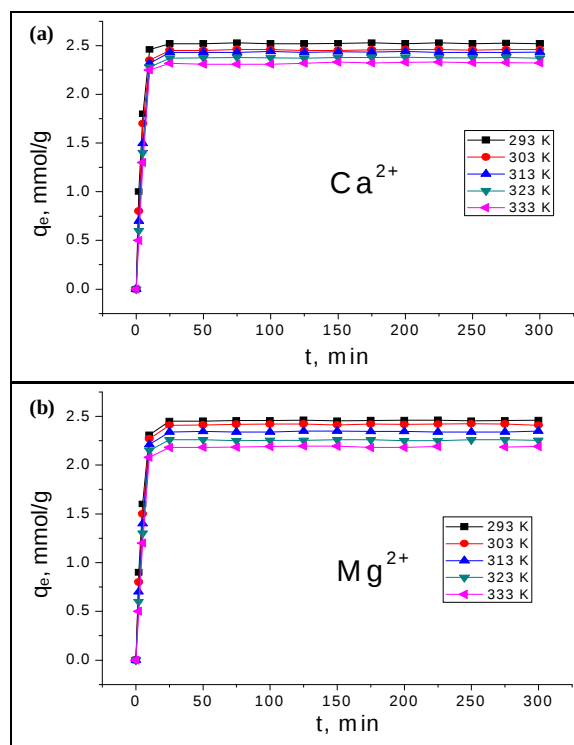
Figure 6. Effect of temperature on the adsorption \text{Ca}^{2+} and \text{Mg}^{2+} ions to SPVC resin in the industrial wastewater
