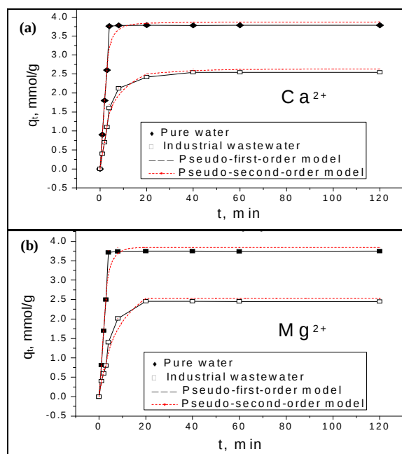
Figure 3. Adsorption kinetics of (a) \text{Ca}^{2+} and (b) \text{Mg}^{2+} ions in pure water and industrial wastewater solution
