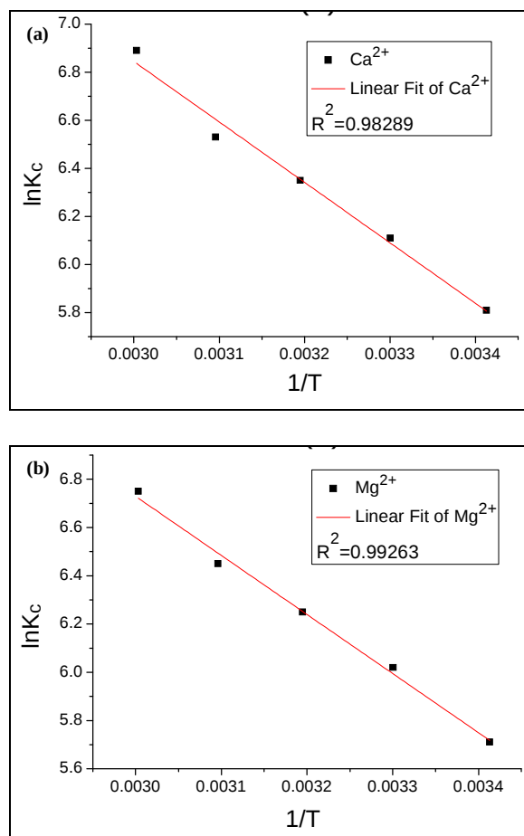
Figure 7. The plot of \ln K_c versus 1/T for \text{Ca}^{2+} and \text{Mg}^{2+} ions
