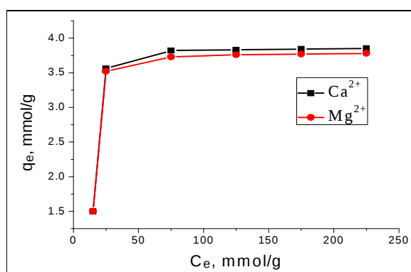
Figure 1. Adsorption isotherms of \text{Mg}^{2+} and \text{Ca}^{2+} ions in pure water
