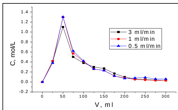
Figure 5. Elution plots of the metal ions
