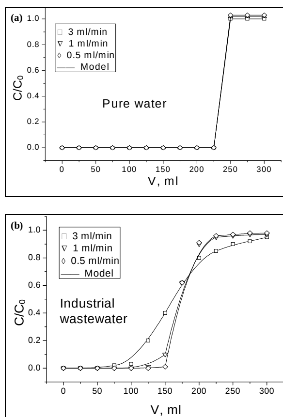
Figure 4. Breakthrough nature of the metal ions in (a) pure water and (b) industrial wastewater
