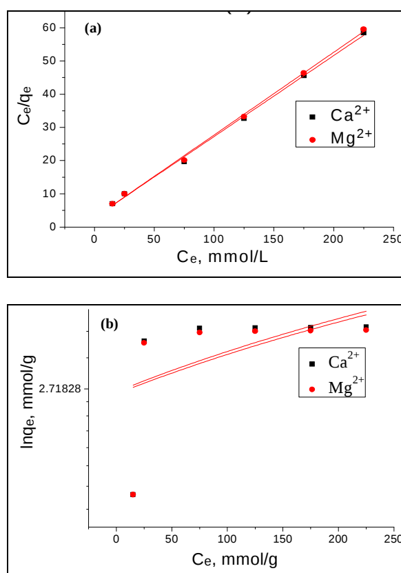
Figure 2. (a) Langmuir and (b) Freundlich adsorption isotherms for \text{Mg}^{2+} and \text{Ca}^{2+} ions in the pure water
